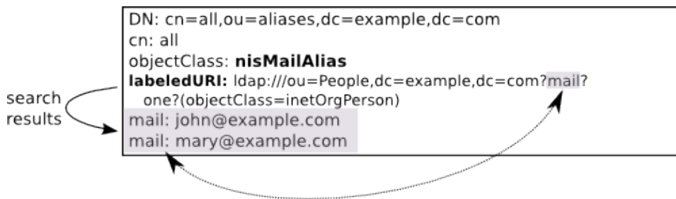
Figure X.Y: Dynamic List for all emails
